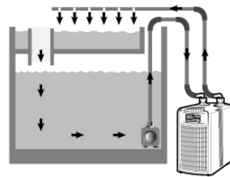
3. Connection of inside circulation pump
