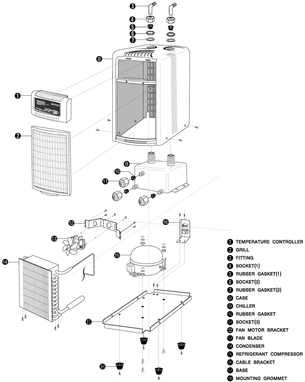
Figure 3 Exploded View and Part List
